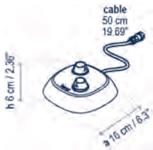
Birdie Base 2 Conexiones / Birdie Base 2 Connections
