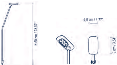
Birdie Luminaria 60SC / Birdie Luminaire 60SC
